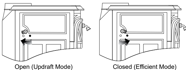
Figure 2.3 - The damper is either open or closed. There are no intermediate positions.
