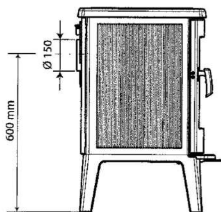
Rear connection
