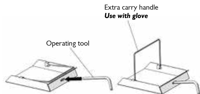
Fig. 3 Ashpan removal
