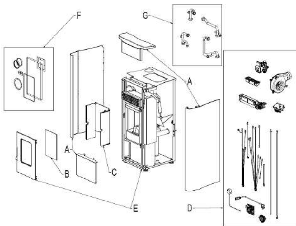
Fig. 1 - Exploded drawing
