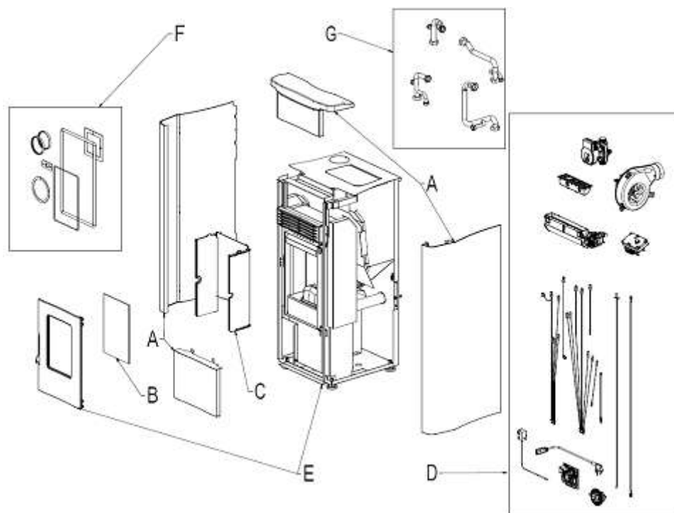
Fig. 1 - Exploded drawing
