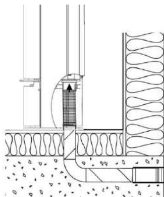
Through floor and foundation
