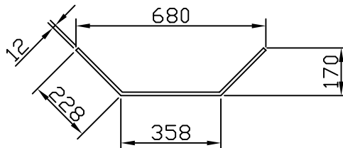
Doorsnede kader Grundriss Blende Coupe Crosssection trim
